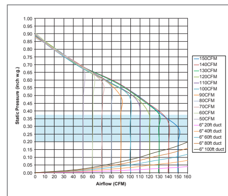
FV-15NLF51 50-150 CFM 6" Duct
